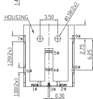
PIN DEFINE
