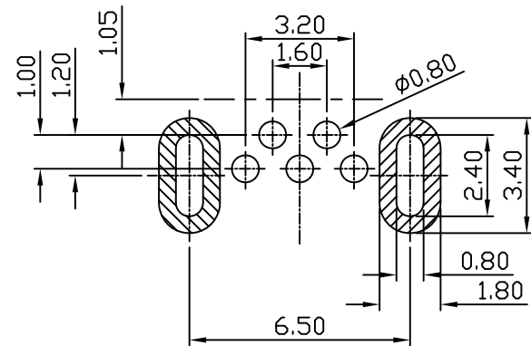
HOLE LAYOUT (TOP VIEW)
